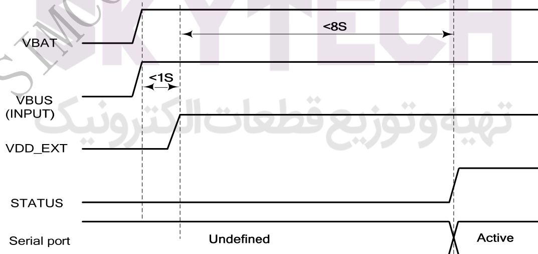
Figure 13: Timing of power on module
