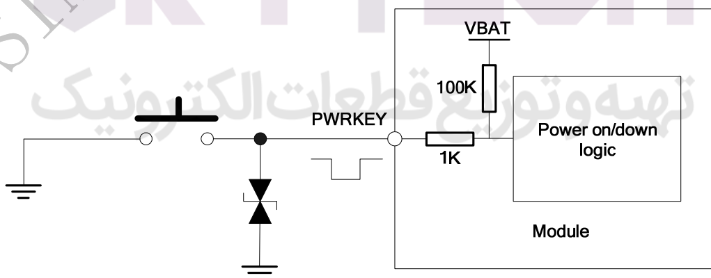
Figure 11: Powered on/down module using button
